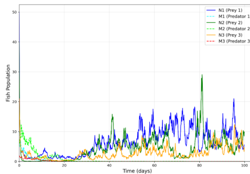
Figure 3: Moderate noise ( \sigma_{N1} = 0.45, \sigma_{M1} = 0.40, \sigma_{N2} = 0.50, \sigma_{M2} = 0.45, \sigma_{N3} = 0.55, \sigma_{M3} = 0.50 ). Pronounced oscillations but persistence.
