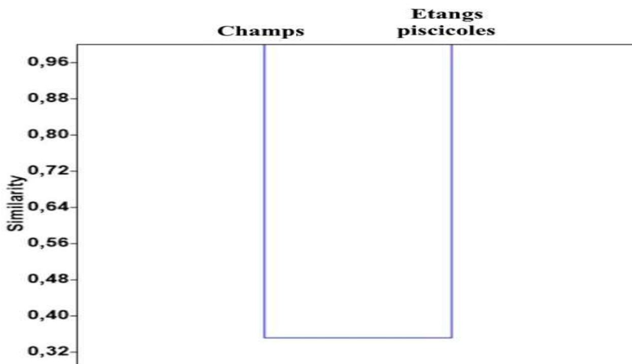
Figure 2 Similarity Dendrogram
